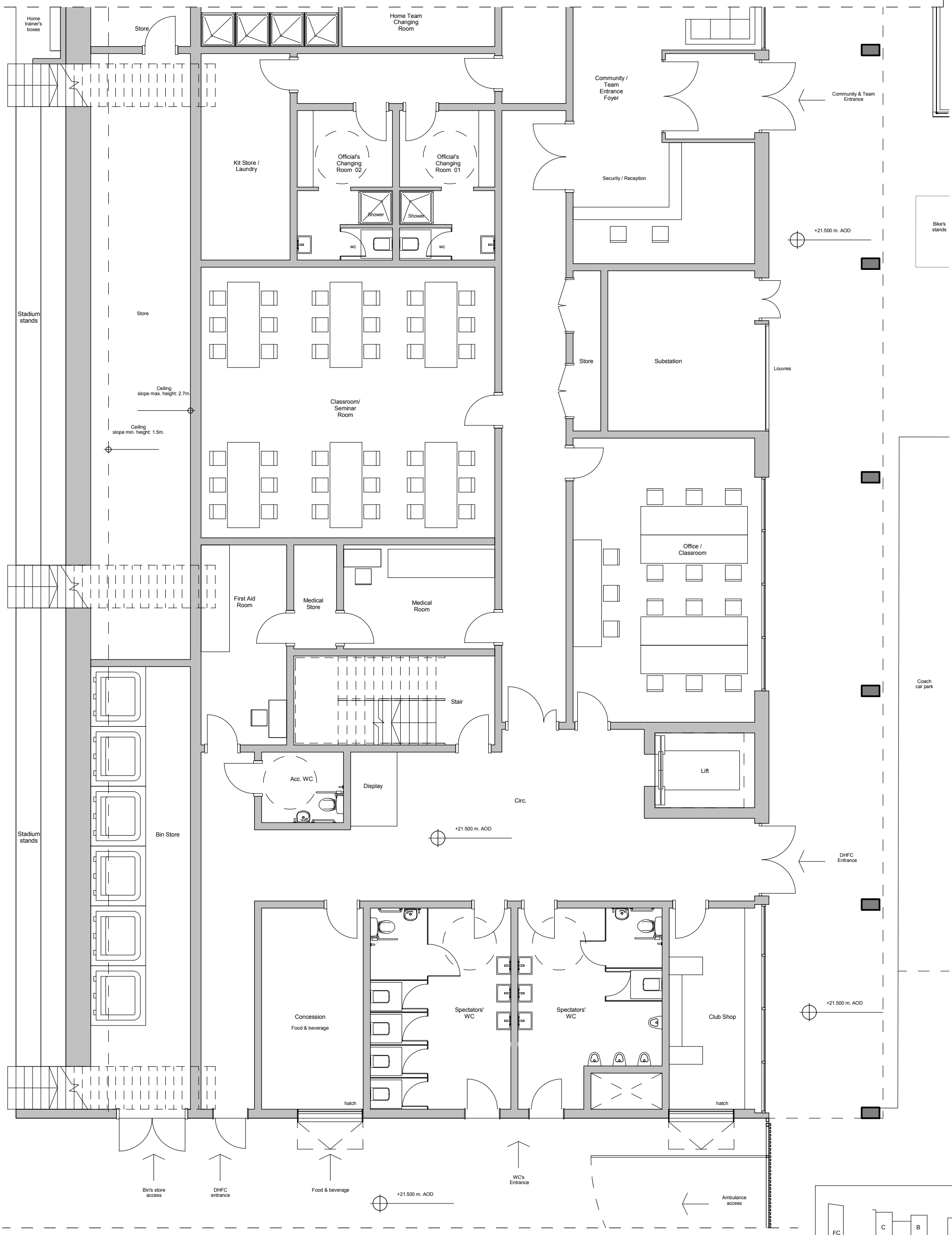
1 PA-05-150 Football Club - Stadium Ground Floor - South SCALE 1 : 100
