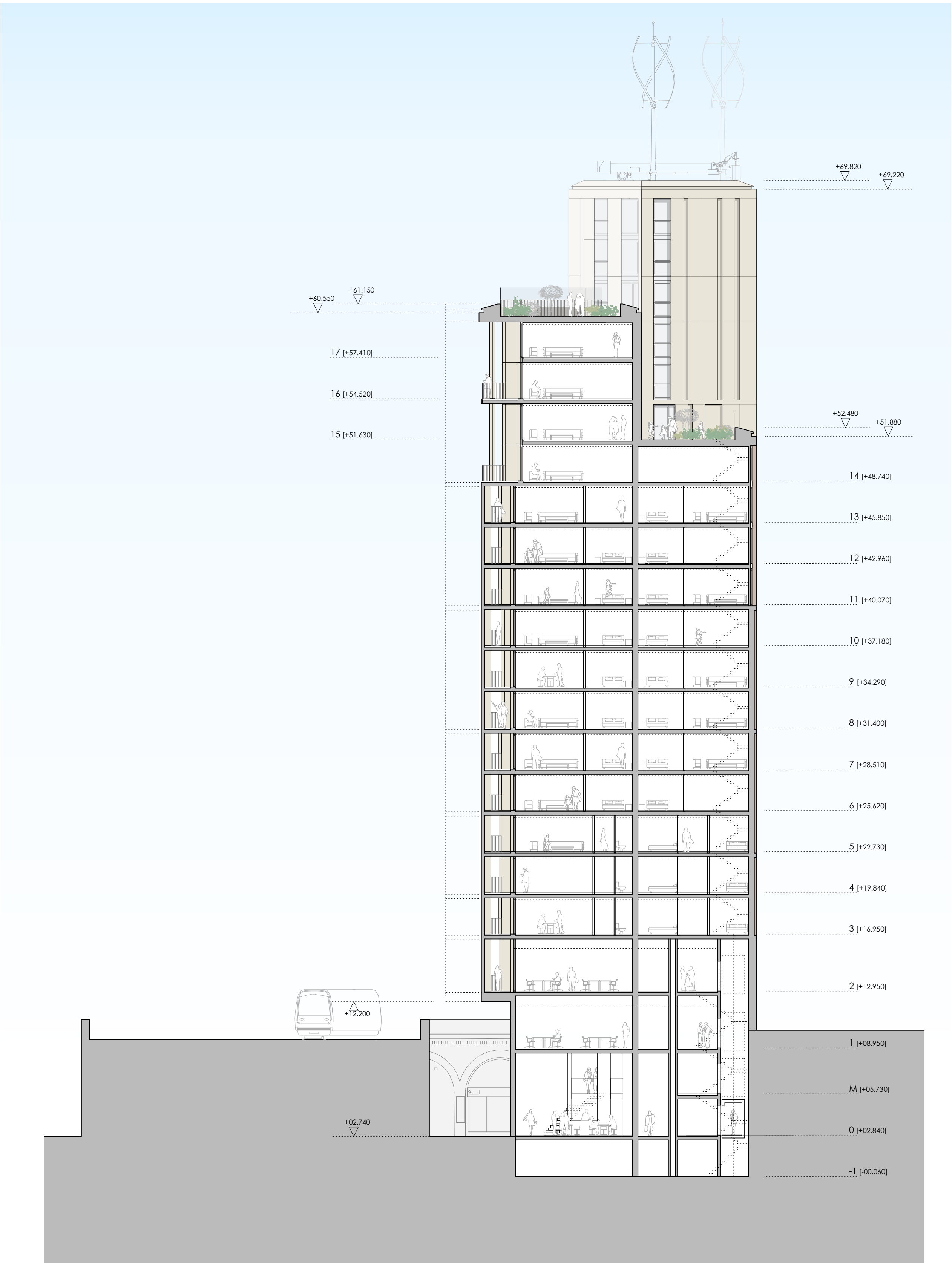
SECTION BB / PENTHOUSE ELEVATION C / 1:200
