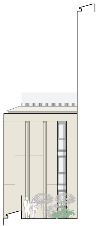
PENTHOUSE ELEVATION D
